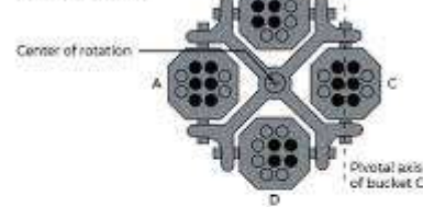
Balanced Load Top View of Partially-Filled Rotor
